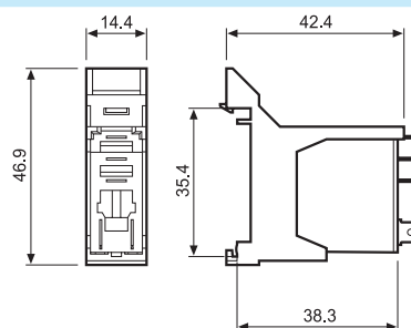
046.07 with relay
