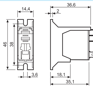
046.05 with relay
