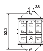
062.05 with relay
