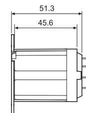
062.05 with relay
