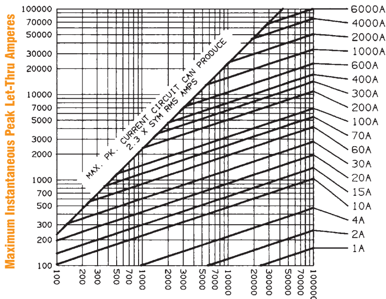
Peak Let-Thru Current Data – A13X1 to 6000, 130 Volts AC
