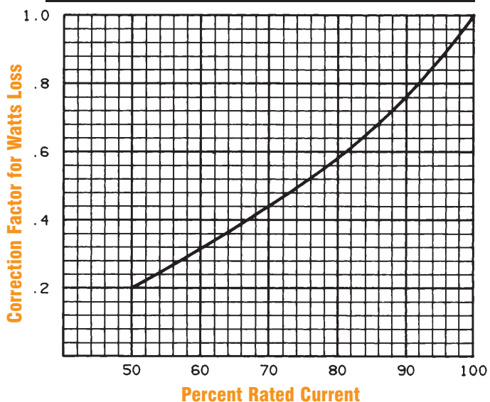
Watts Loss Correction vs. Percent Rated Current
