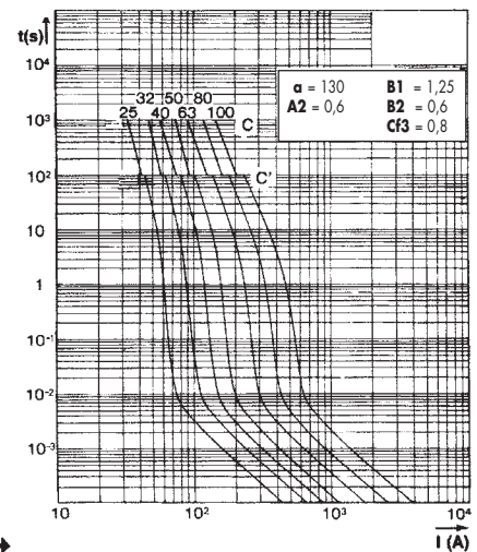
A70QS25 to 100 (22F, 22FI)
