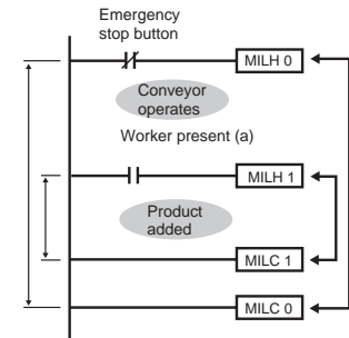
CX-Programmer Screen
