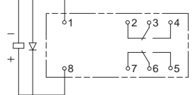
G2R-2-SN (S), G2R-2-SNI (S) (DC)
