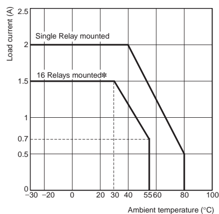
G3R-OA202SN□N
