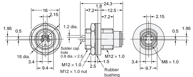
XS3P-M421-2 (Solder Cup Pins)
