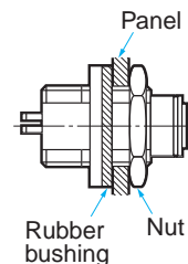
Front Lock
