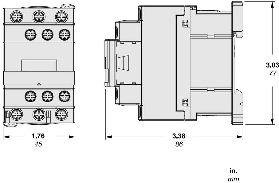
CONTACTOR WITH DC COIL
