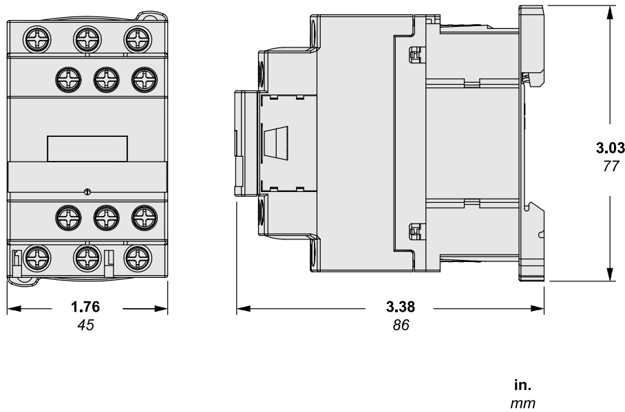
CONTACTOR WITH DC COIL
