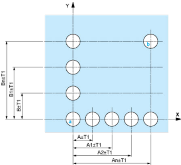
Panel Cut-outs (Viewed from Installer's Side)
