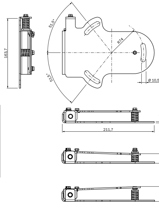
Dimensional drawing
