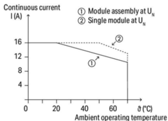
Current-carrying capacity curve
