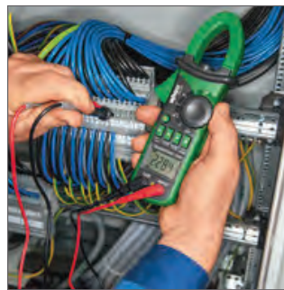
Meter utilizing test probes for voltage measurement
